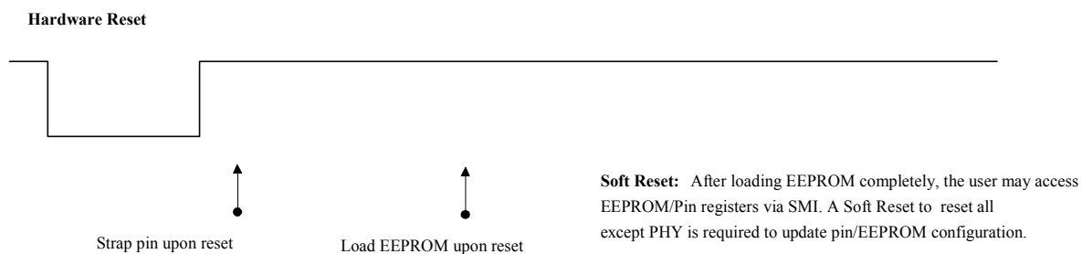
Figure 4. Reset
