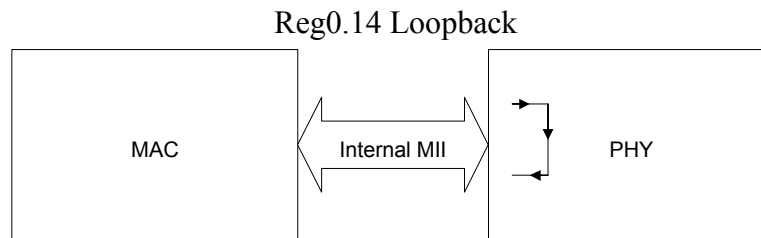
Figure 15. Reg. 0.14 Loopback
