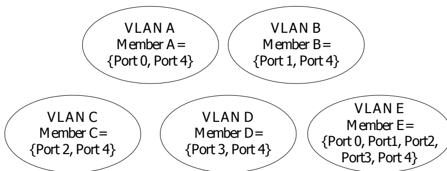
Figure 9. VLAN Configuration
