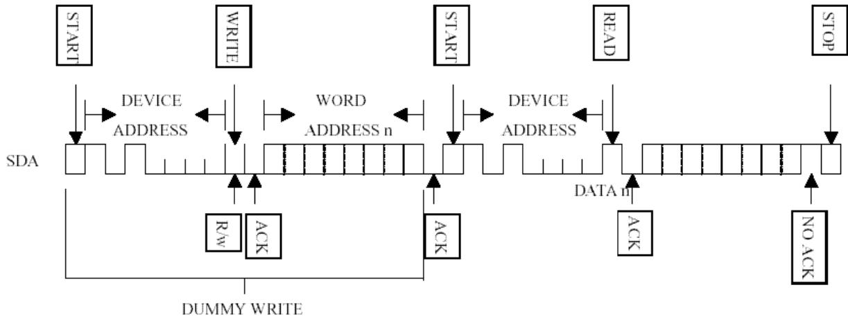
Figure 7. Random Read
